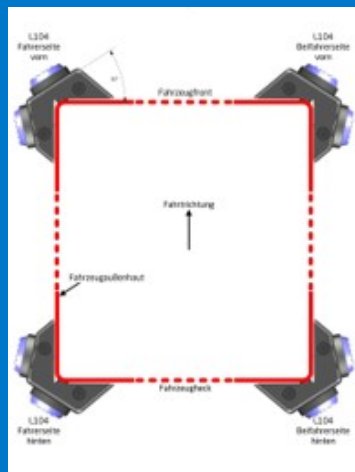
corner mounting
